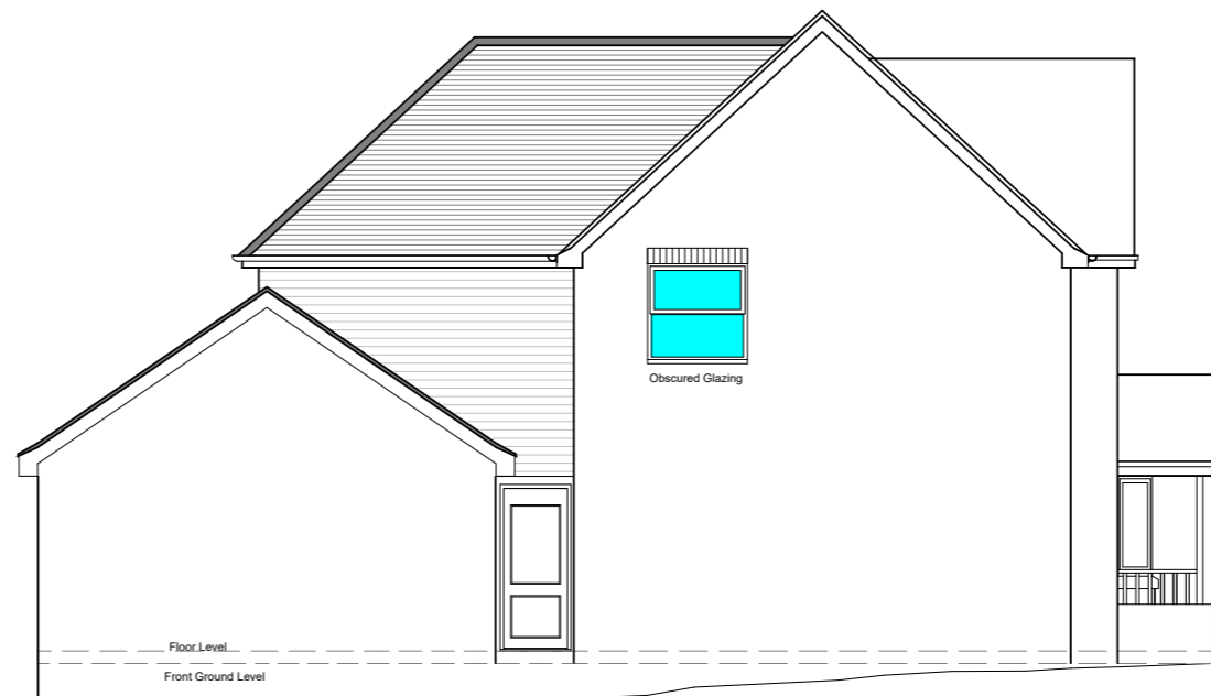
Proposed L/H Side Elevation
