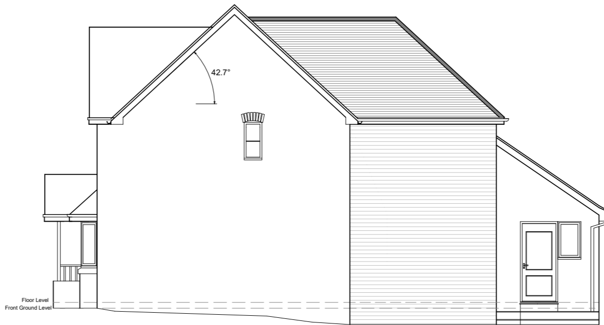
Proposed R/H Side Elevation
