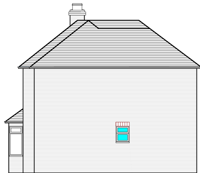
Proposed RH side Elevation
