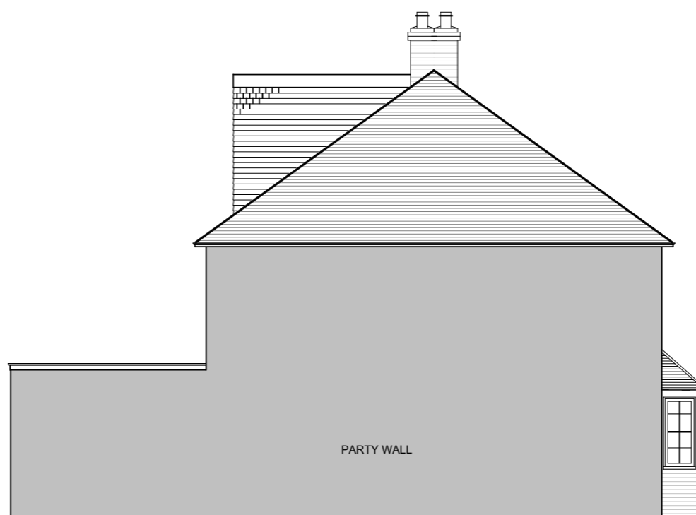
Proposed LH Side Elevation
